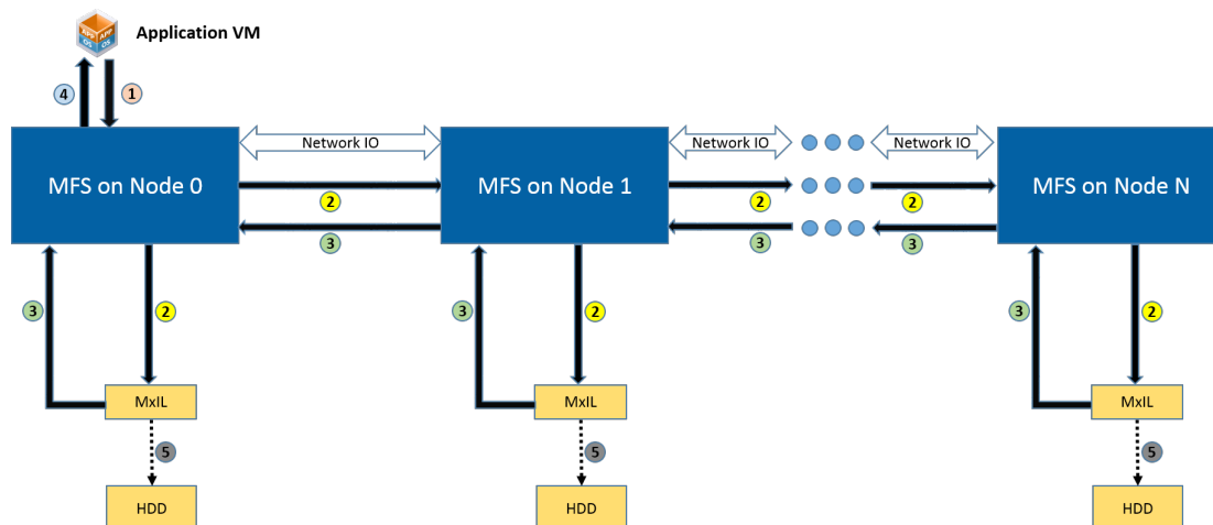
Figure 4: MxSP Write I/O Path
