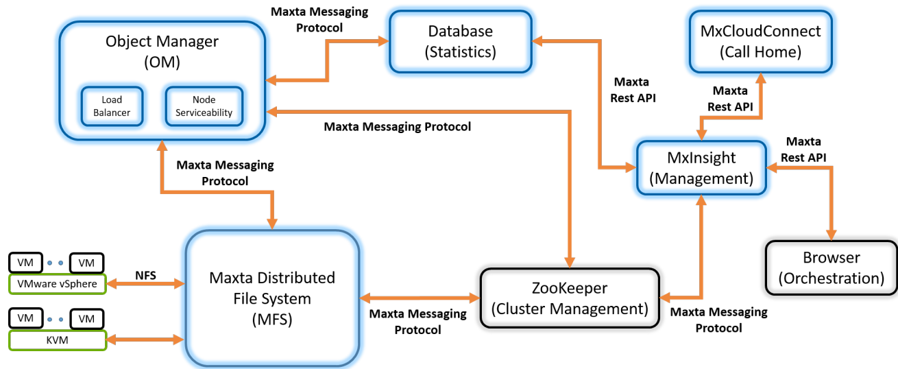
Figure 3: MxSP Component Relationship
