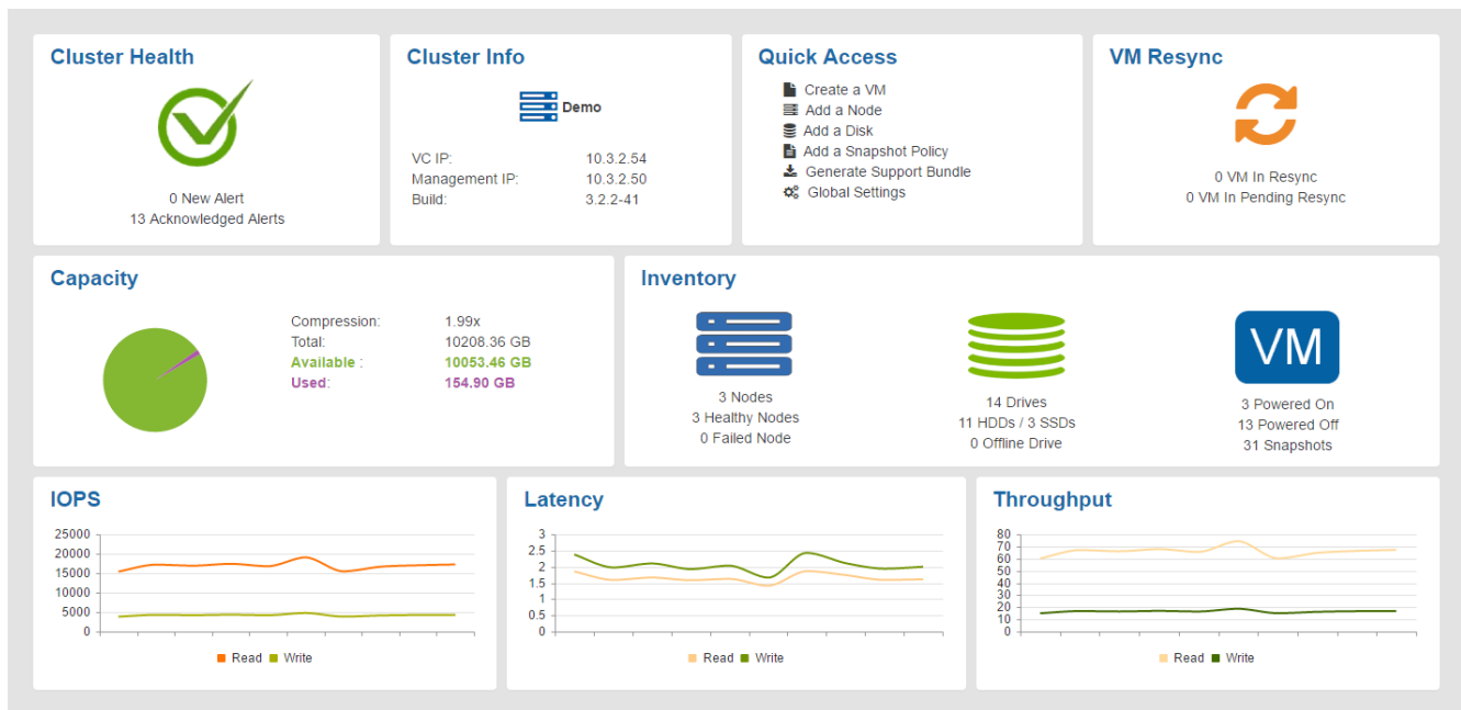
Figure 35: MxInsight Dashboard
