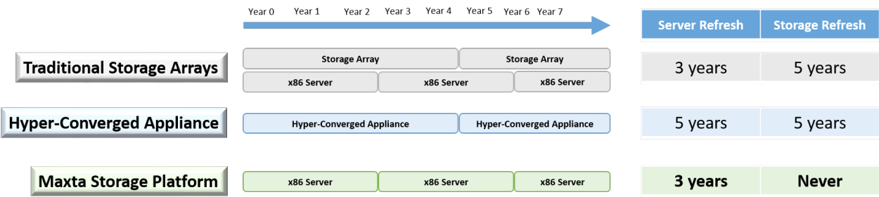
Figure 52: Software Agility
