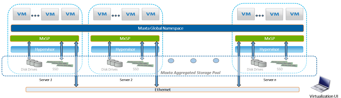
Figure 1: MxSP Architecture
