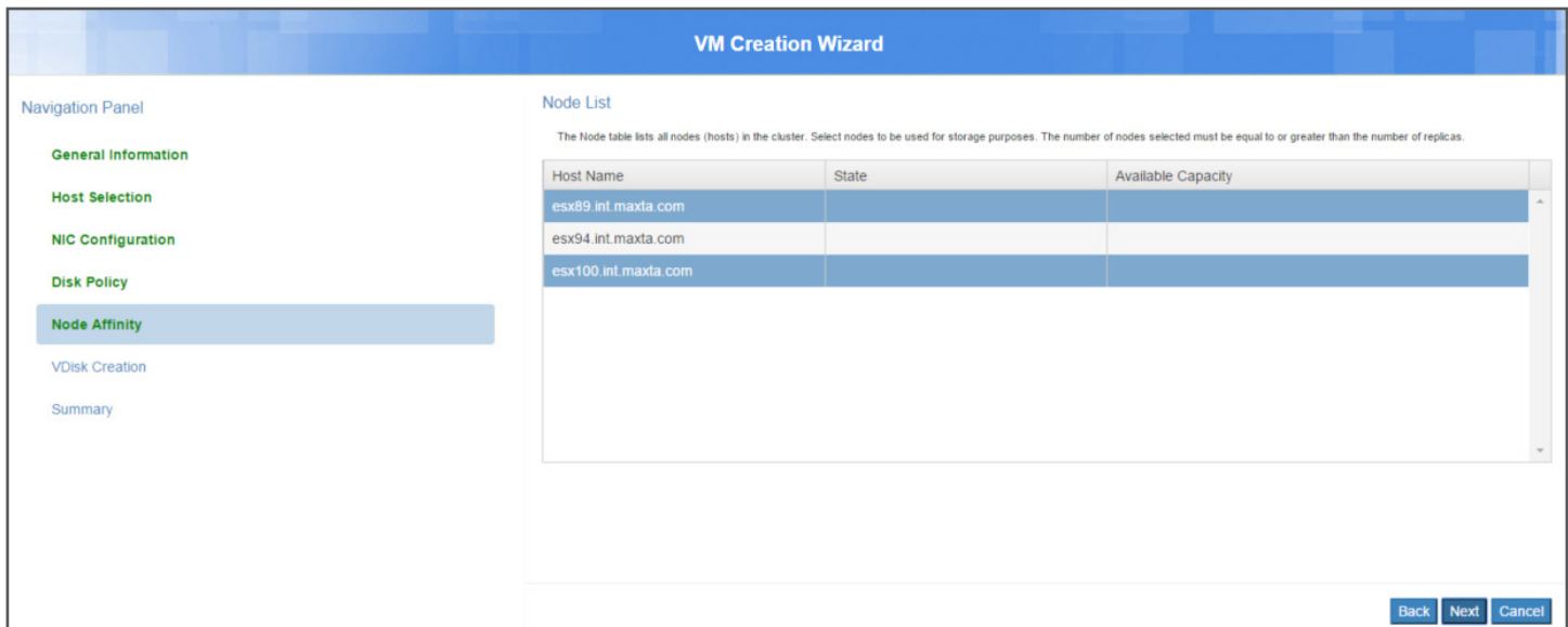
Figure 29: Node Affinity
