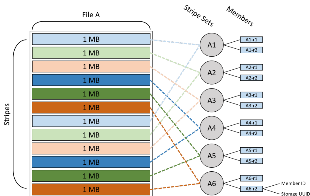
Figure 13: Data Striping
