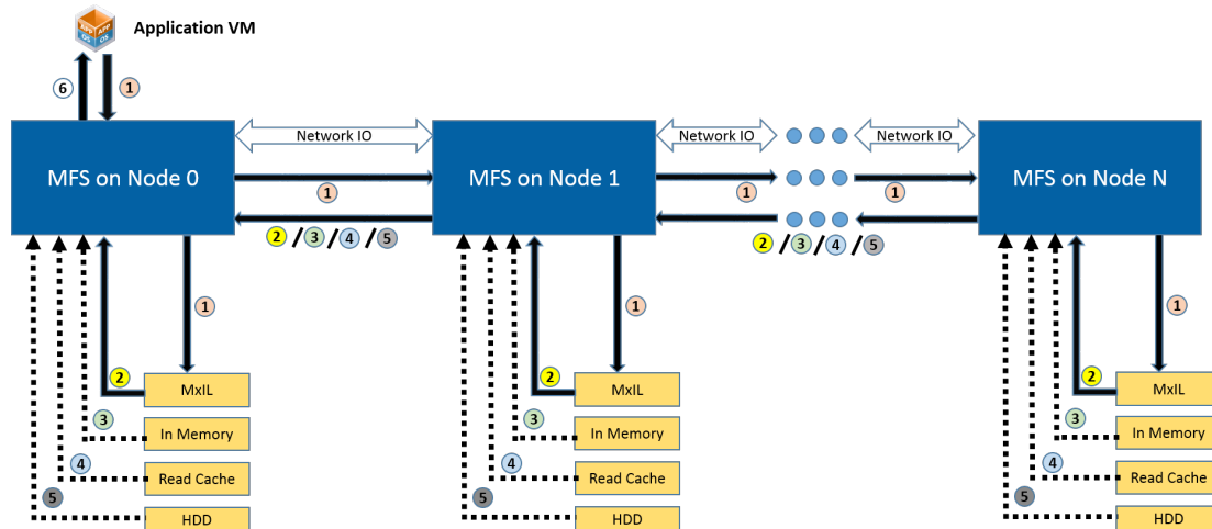
Figure 5: MxSP Read I/O Path
